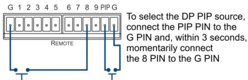
Figure 35: Connecting the PIP Contact Closure Remote Control PINs
