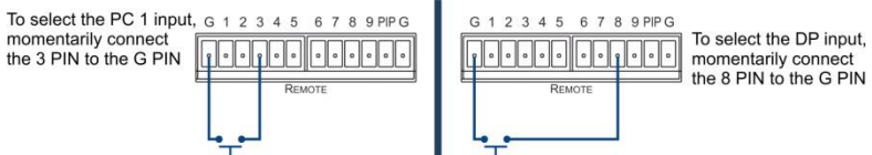
Figure 34: Connecting the Contact Closure Remote Control PINs
