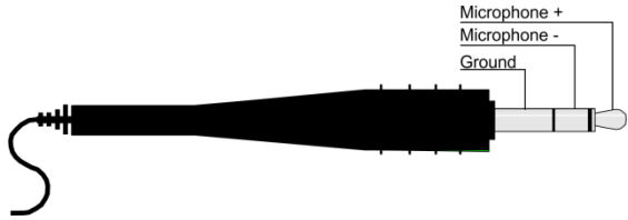
Figure 6: Microphone Pinout
