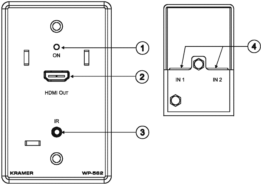
Figure 6: WP-562 HDMI Line Receiver US Model Functions
