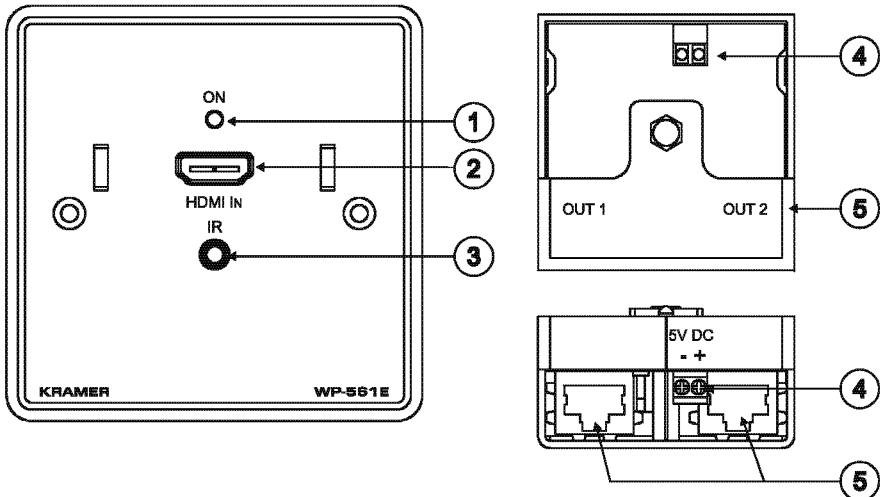
Figure 2: WP-561 HDMI Line Transmitter UK/European Model Functions
