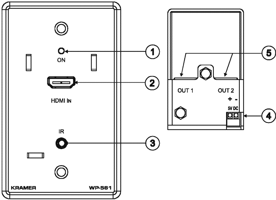
Figure 3: WP-561 HDMI Line Transmitter US Model Functions
