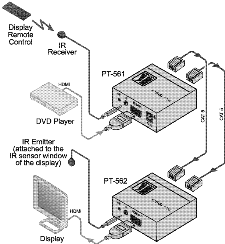
Figure 9: Connecting the PT-561/PT-562 HDMI Line Transmitter/Receiver
