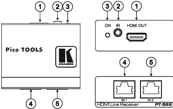
Figure 8: PT-562 HDMI Line Receiver
