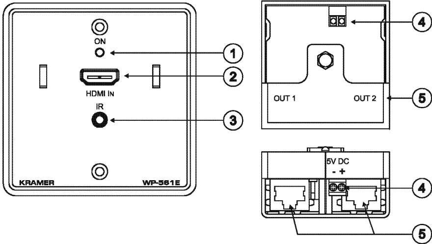
Figure 1: WP-561 HDMI Line Transmitter Belgian/German Model Functions
