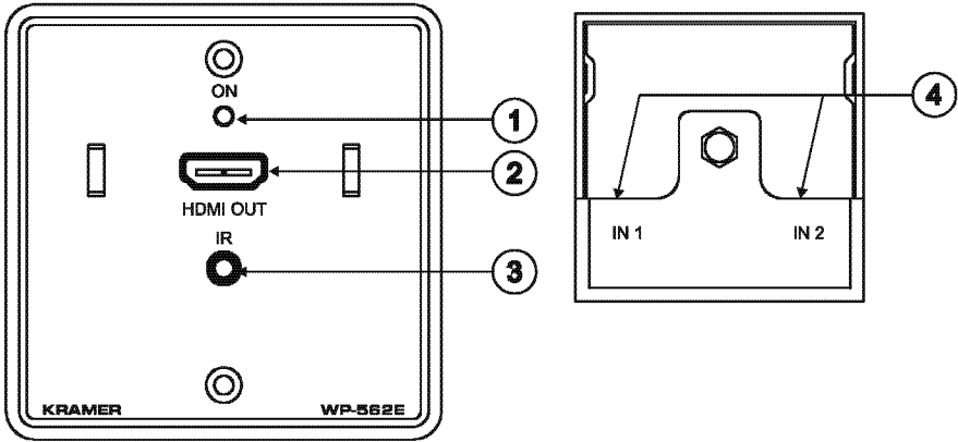
Figure 4: WP-562 HDMI Line Receiver Belgian/German Model Functions
