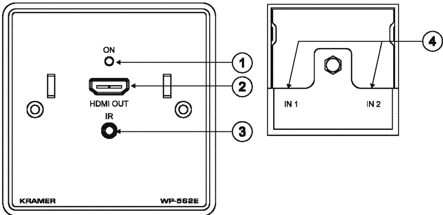
Figure 5: WP-562 HDMI Line Receiver UK/European Model Functions
