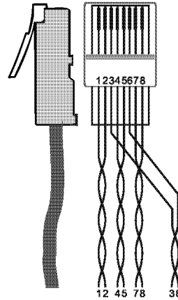
Figure 10: CAT 5 PINOUT
