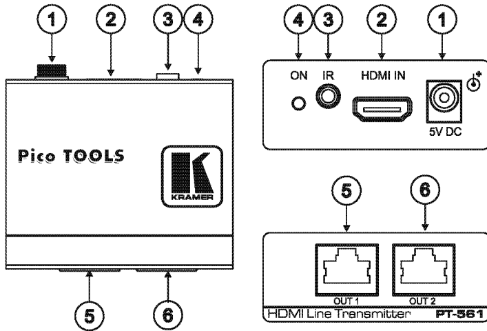
Figure 7: PT-561 HDMI Line Transmitter
